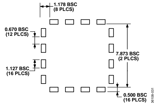
Figure 35. Example Pad Layout
