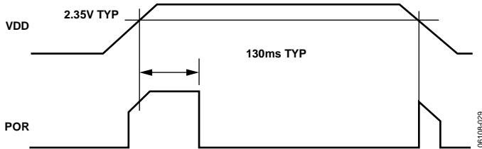
Figure 33. Internal Power-On Reset Operation
